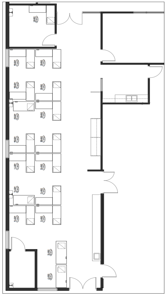
1 FURNITURE PLAN - CATEGORIES 1, 2 & 5 PLAN DU MOBILIER - CATEGORIES 1, 2 ET 5 SCALE = 1:50 ECHELLE = 1:50
